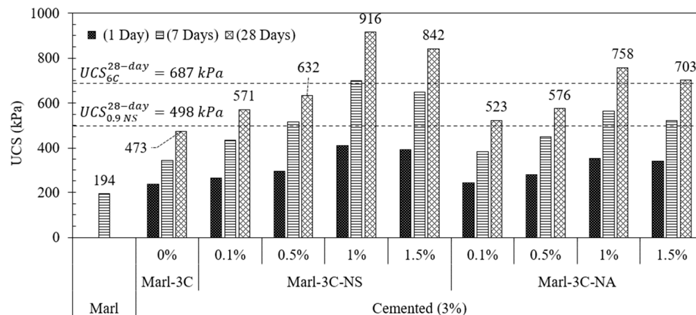
Figure 3. Unconfined compressive strength of stabilized marl.
