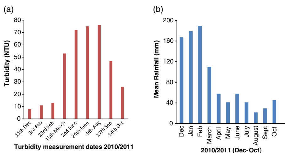
Figure 8 (a) Turbidity measurements of un-filtered pond water of the CQUniversity aquaculture system, starting from Dec, 2010 –Oct 2011. (b) Mean rainfall (mm) in Dec, 2010/Oct, 2011- data obtained from Bureau of Meteorology, Government of Australia.
