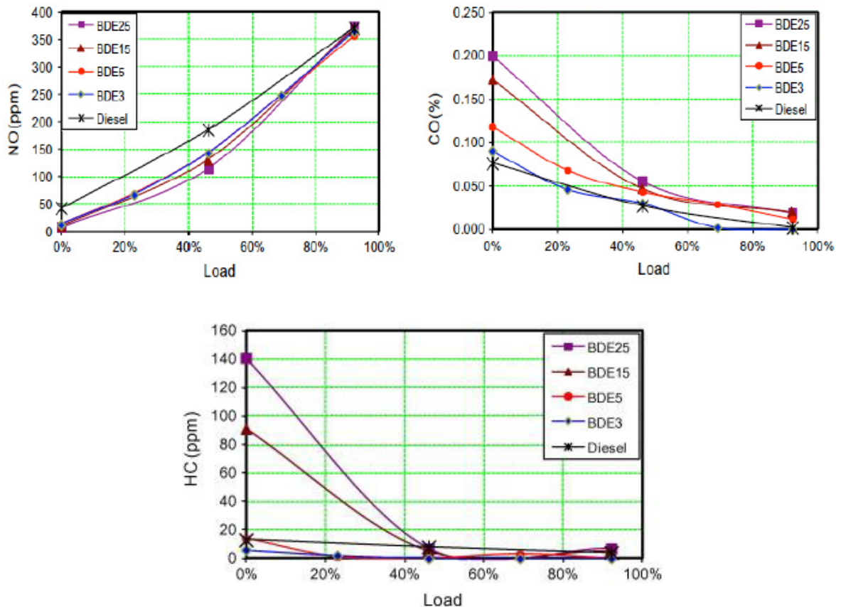
Fig. 1: Effect of diesel-biodiesel-ethanol blends on NO, CO and HC [11]
